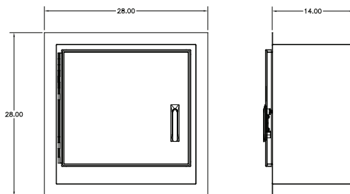
Recessed
